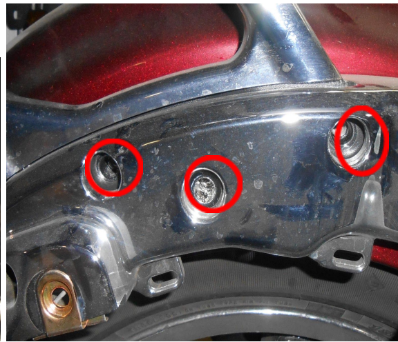
Step 8- Bolt Positions Seen on Right Side of Motorcycle- Rearmost Bolt Position not used for hitch Installation Highlighted
